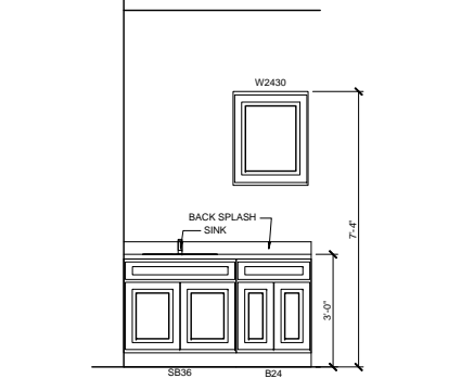
C INTERIOR ELEVATION SCALE: 1/2" = 1'-0"
