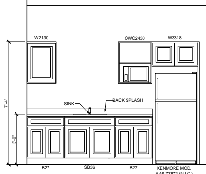
B INTERIOR ELEVATION SCALE: 1/2" = 1'-0"
