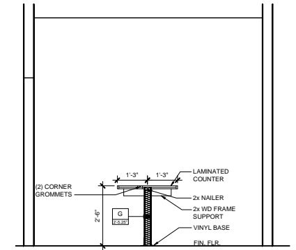
A INTERVIEW DESK SECTION SCALE: 1/2" = 1'-0"
