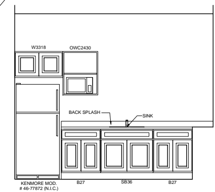
D INTERIOR ELEVATION SCALE: 1/2" = 1'-0"
