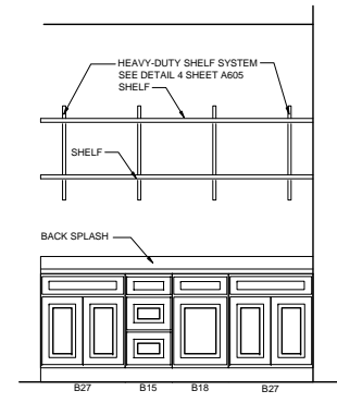
3 INTERIOR ELEVATION SCALE: 1/2" = 1'-0"
