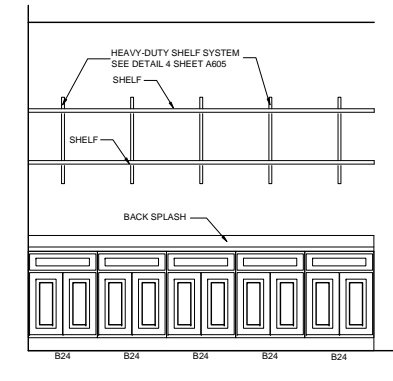
6 INTERIOR ELEVATION SCALE: 1/2" = 1'-0"
