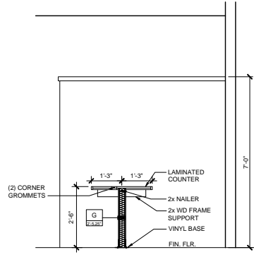
4 INTERIOR ELEVATION SCALE: 1/2" = 1'-0"
