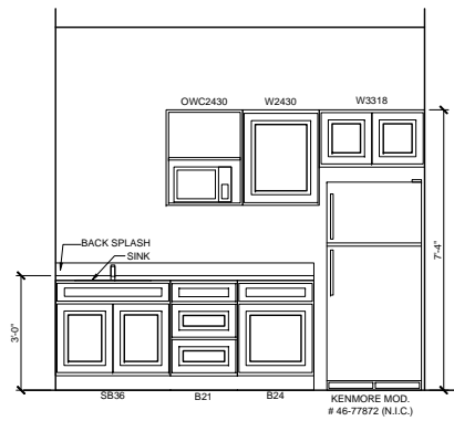
2 INTERIOR ELEVATION SCALE: 1/2" = 1'-0"
