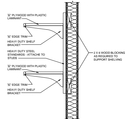
4 TYPICAL HEAVY DUTY SHELF SYSTEM SCALE: 1 1/2" = 1'-0"
