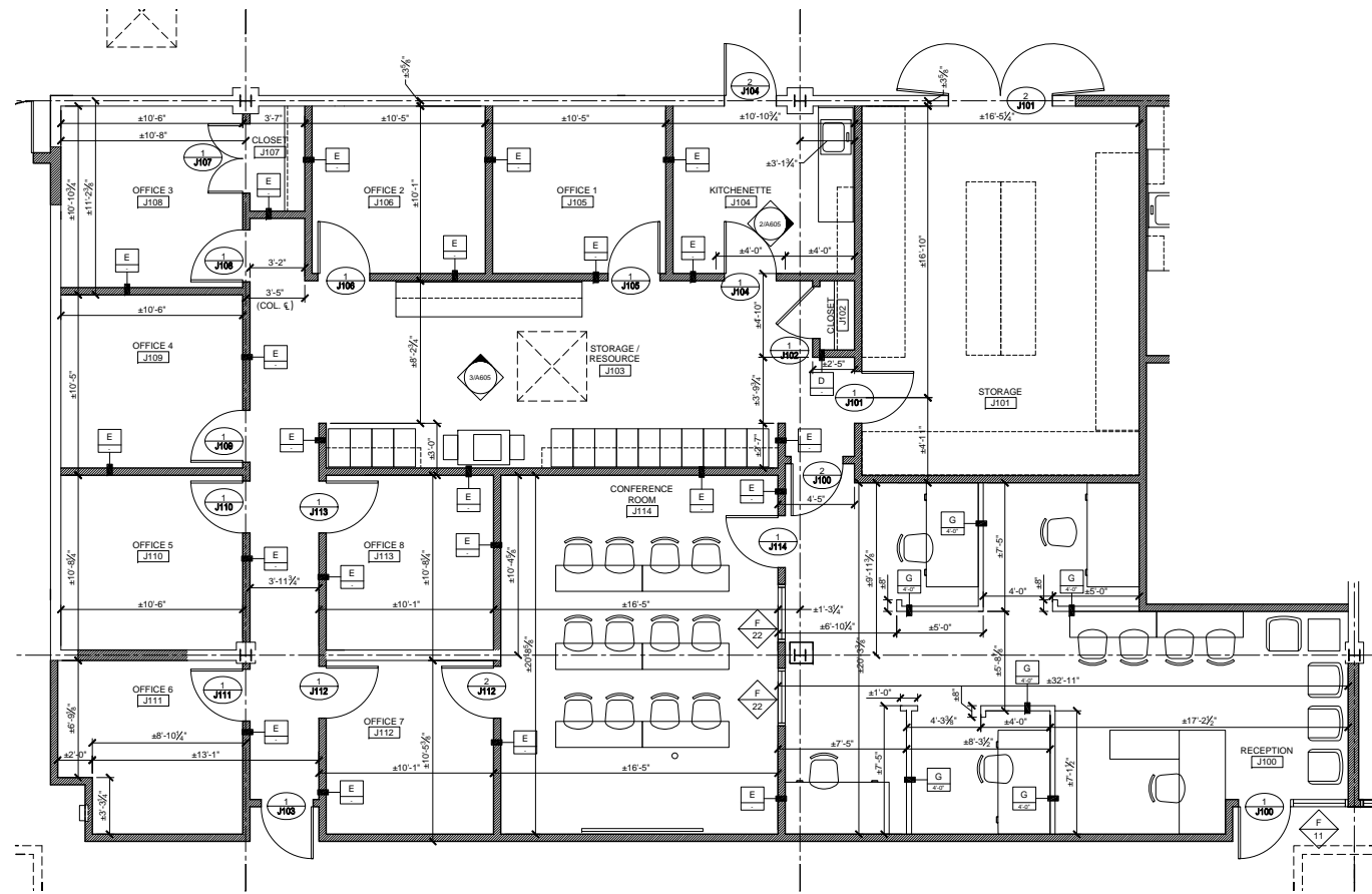
1 TELAMON SPACE PLAN SCALE: 1/4" = 1'-0"
